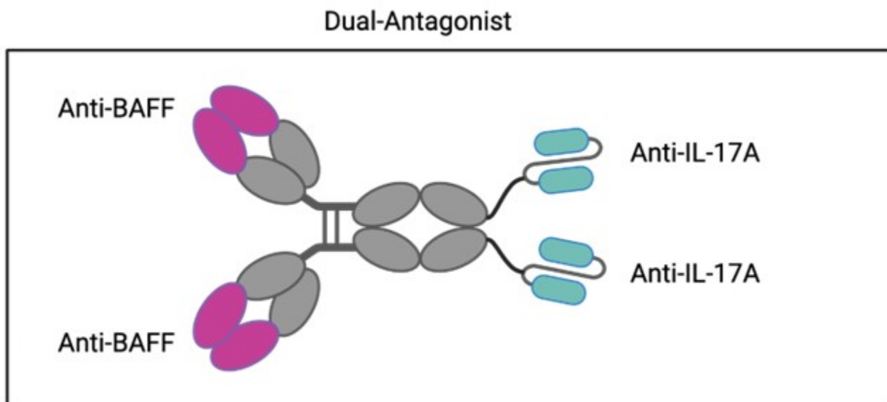
Figure 2: Tibulizumab
